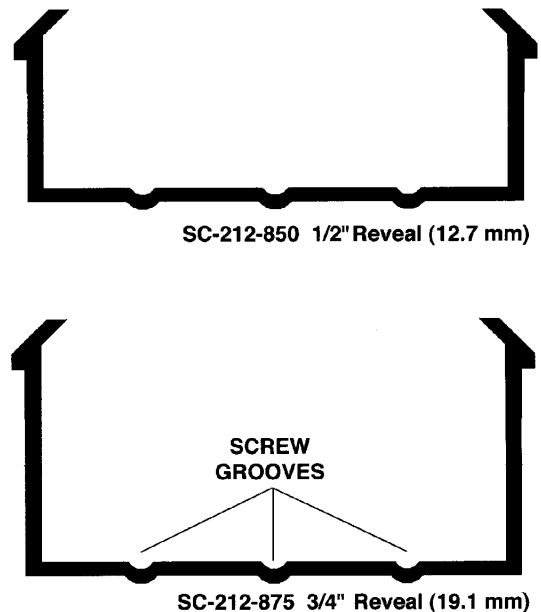
SSB-212-8 SNAP-ON BULLNOSE W/CLIP MOUNTS NO SCALE SECTIONS
